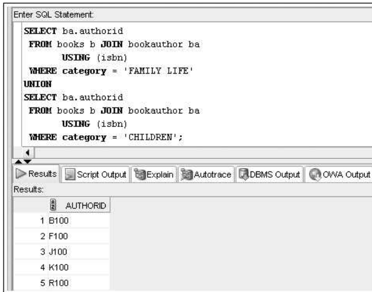
FIGURE 9-31 Producing an unduplicated combined list with the UNION set operator
