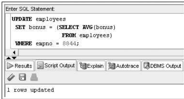
FIGURE 12-29 An UPDATE statement using a subquery
