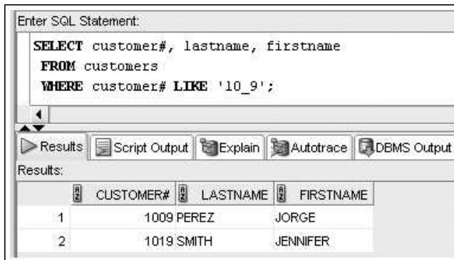
FIGURE 8-20 Searching with the LIKE operator and the _ wildcard character
