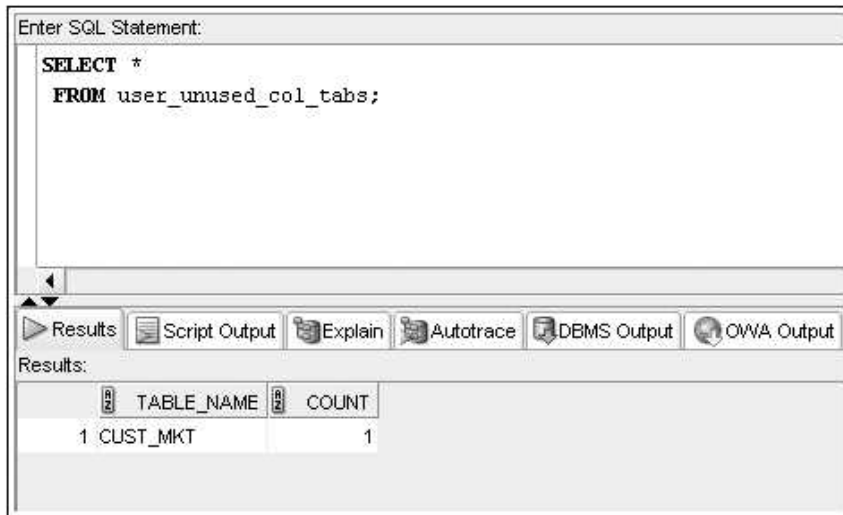
FIGURE 3-29 Listing tables with columns marked as unused
