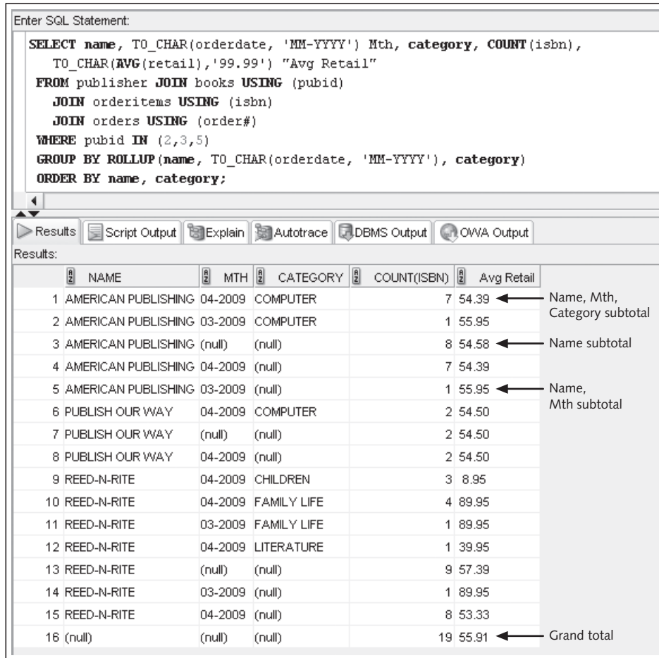
FIGURE 11-39 Using three columns in a ROLLUP operation
