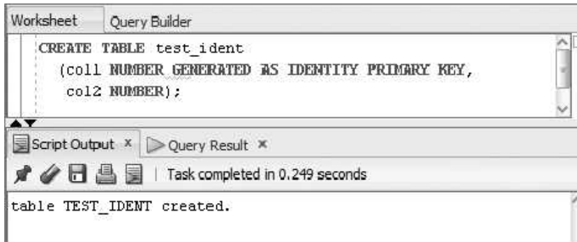
FIGURE 6-21 Create table with an Identity Column
