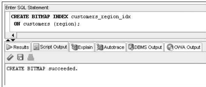
FIGURE 6-31 Creating a bitmap index on the Region column
