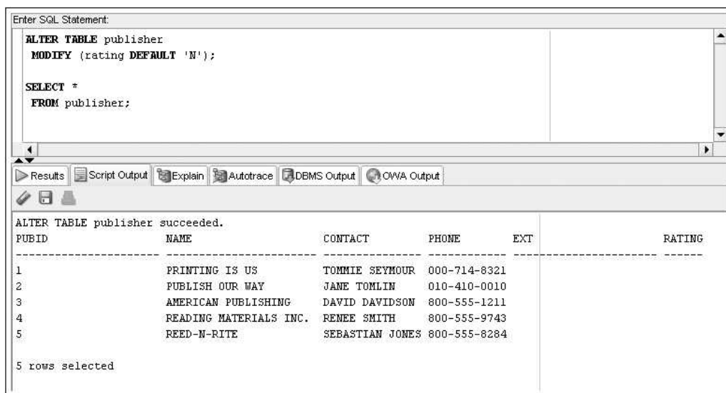
FIGURE 3-21 Adding the DEFAULT option to the new column
