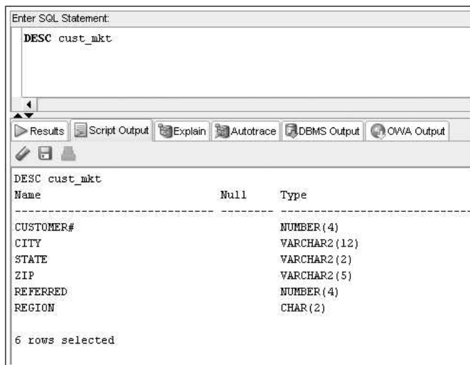
FIGURE 3-12 Using DESCRIBE to verify the new table structure
