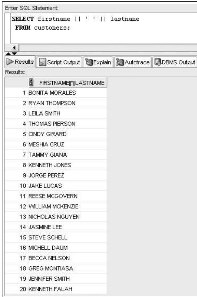
FIGURE 2-19 Using a string literal in concatenation
