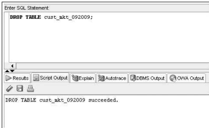
FIGURE 3-38 Using the DROP TABLE command to remove the CUST_MKT_092009 table
