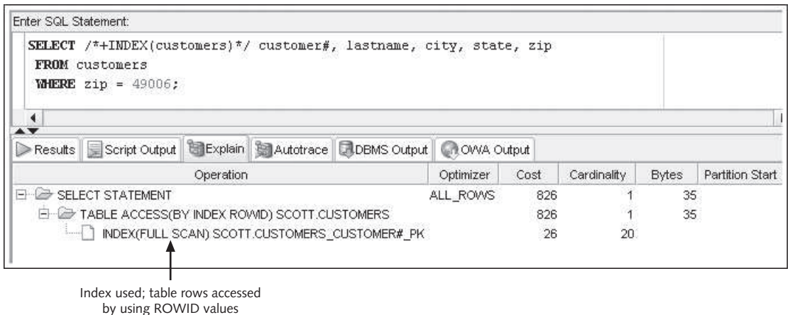
FIGURE 6-27 View the explain plan indicating an index scan
