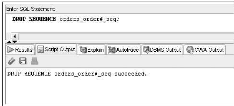
FIGURE 6-19 Dropping the ORDERS_ORDER#_SEQ sequence
