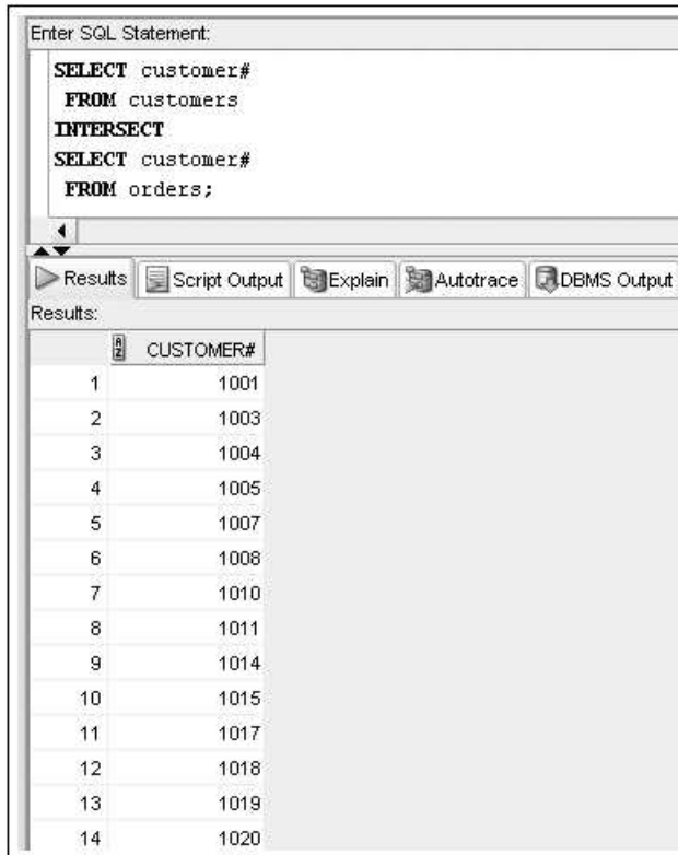
FIGURE 9-37 Identify overlapping values with the INTERSECT set operator
