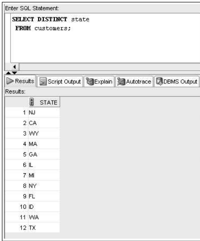
FIGURE 2-16 List of unduplicated states for customers
