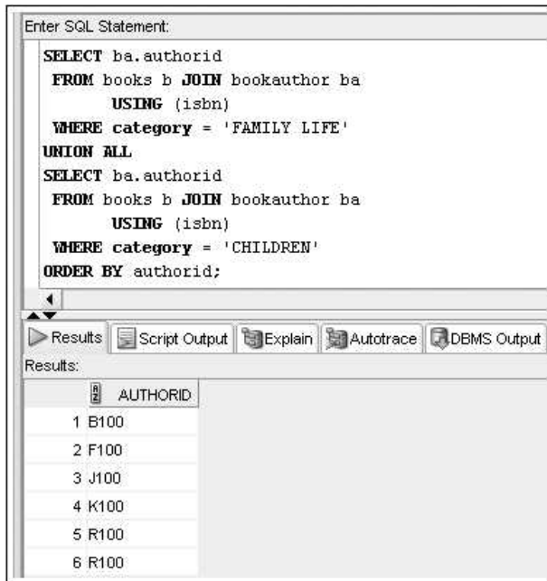
FIGURE 9-33 Add sorting to a set operation
