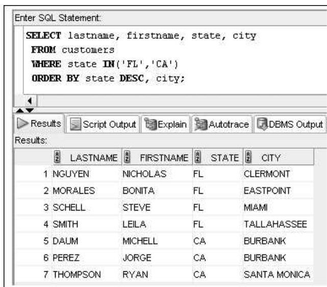
FIGURE 8-39 Sorting on the State and City columns
