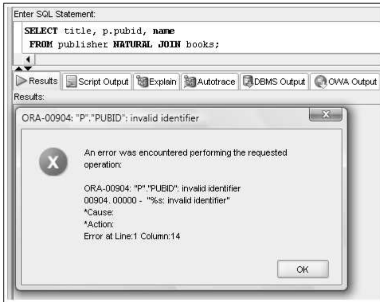
FIGURE 9-13 Column qualifier error with a NATURAL JOIN
