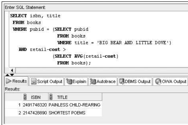
FIGURE 12-6 SELECT statement with two single-row subqueries
