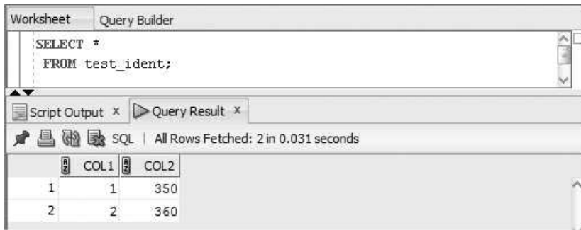
FIGURE 6-23 Columns values resulting from inserts
