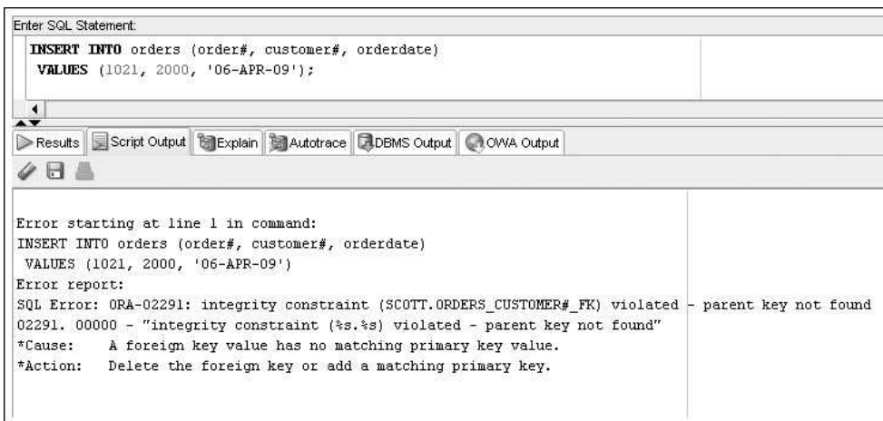
FIGURE 4-10 Insert a row to test the constraint
