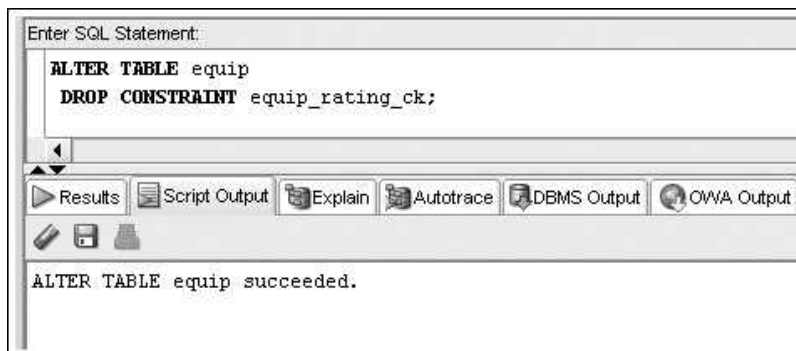
FIGURE 4-38 Dropping a NOT NULL constraint by name
