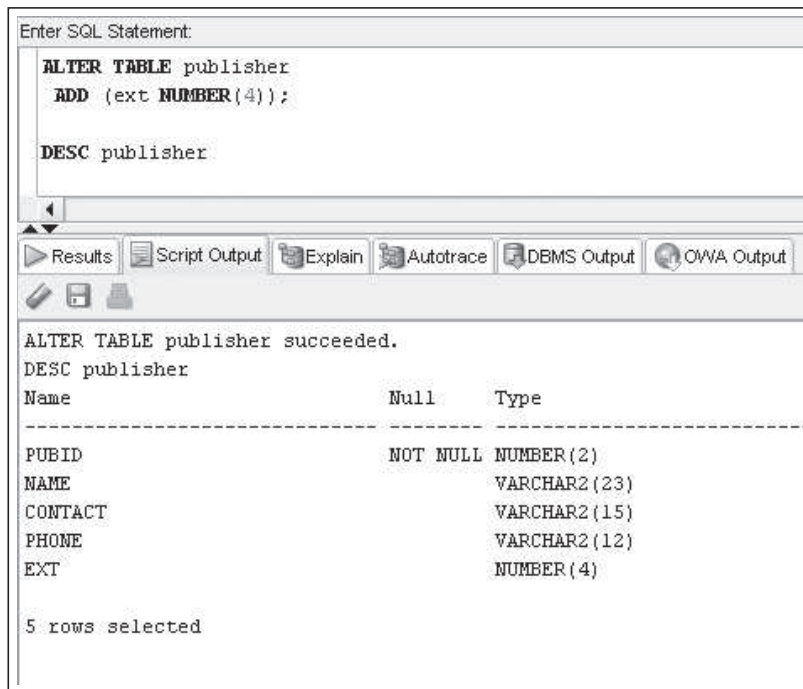
FIGURE 3-16 The ALTER TABLE ... ADD command
