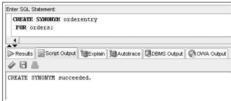
FIGURE 6-43 Create a synonym
