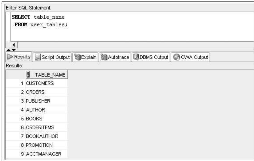
FIGURE 3-3 Listing names of all tables
