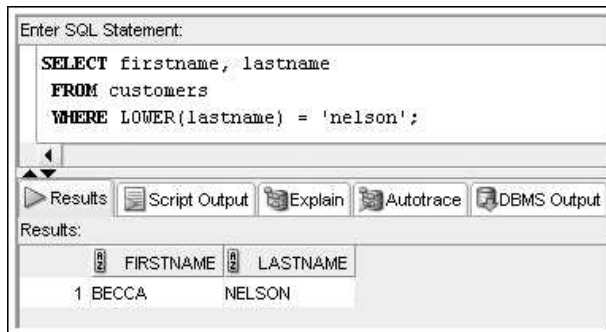
FIGURE 10-1 LOWER function in the WHERE clause
