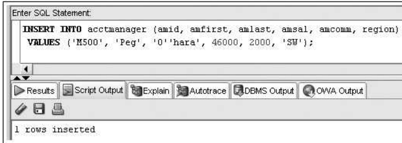
FIGURE 5-18 Use two single quotes in the INSERT value
