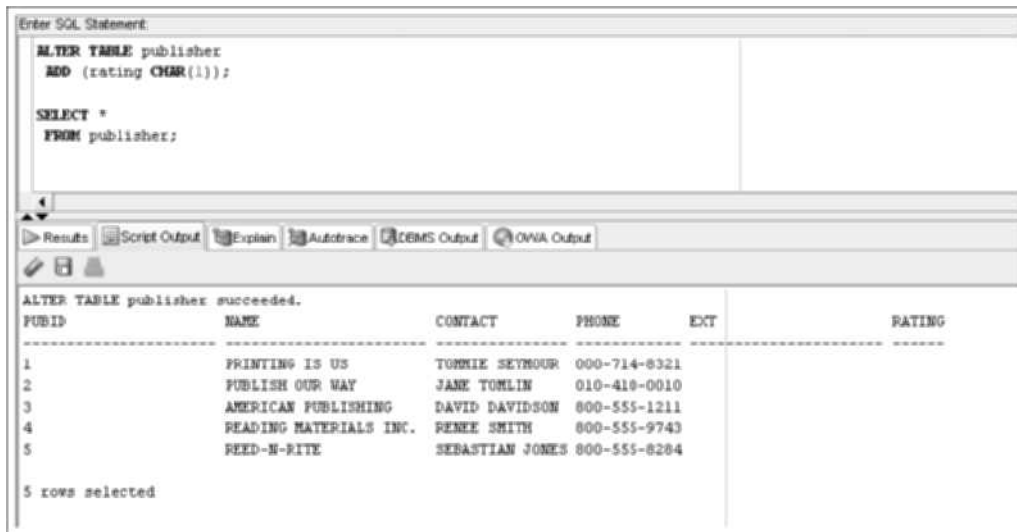
FIGURE 3-20 Adding the Rating column to the PUBLISHER table
