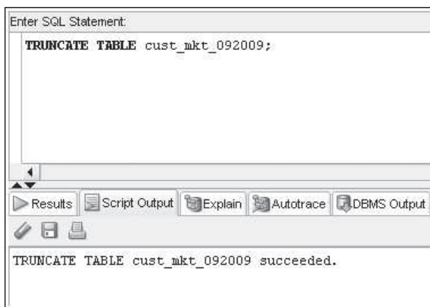
FIGURE 3-36 The TRUNCATE TABLE command
