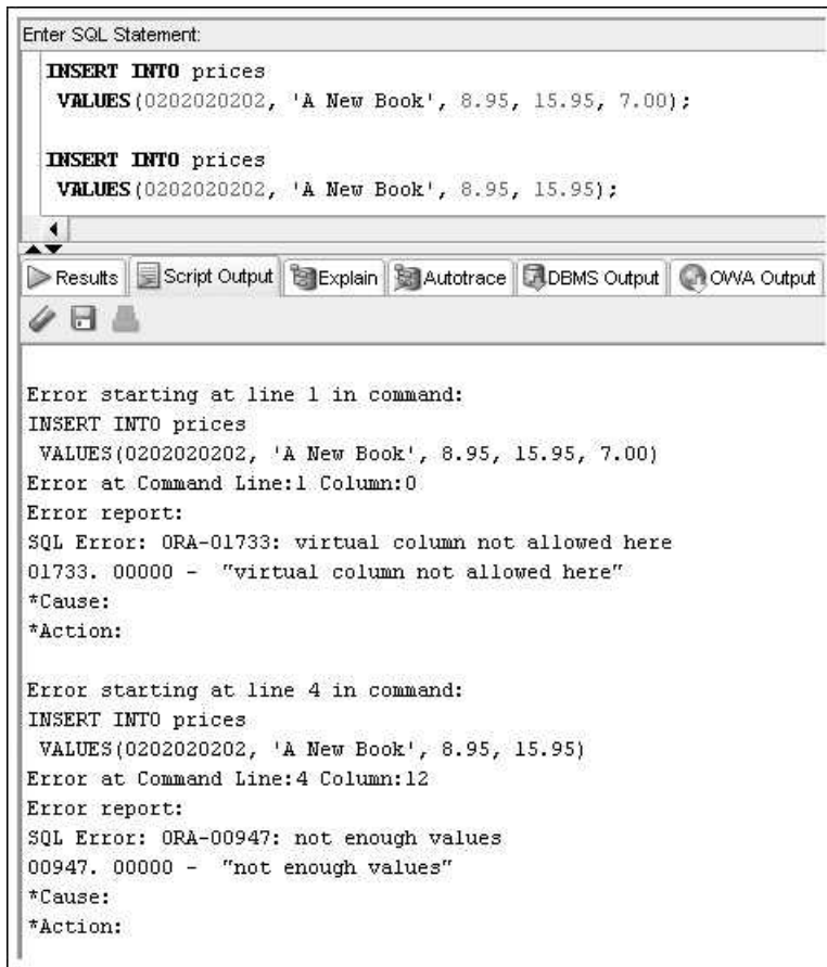
FIGURE 13-14 Failed attempts to add a new book via the PRICES view
