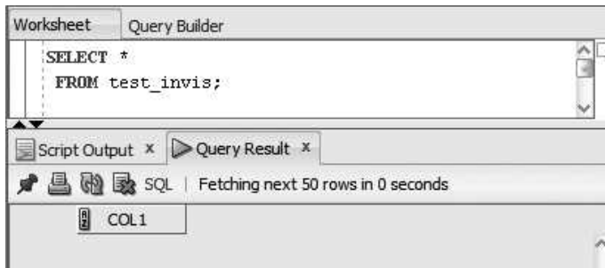
FIGURE 3-7 An invisible column is not shown with a general query
