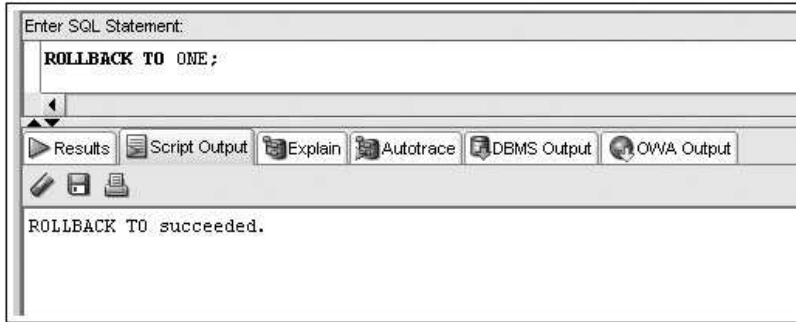
FIGURE 5-38 Undo changes to the SAVEPOINT
