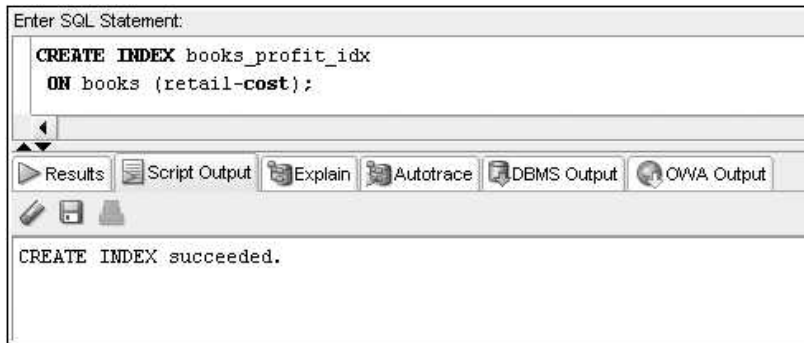
FIGURE 6-33 Creating a function-based index
