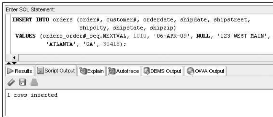
FIGURE 6-6 Inserting a row using a sequence to provide a PRIMARY KEY value
