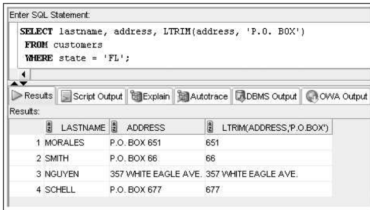
FIGURE 10-12 Using the LTRIM function
