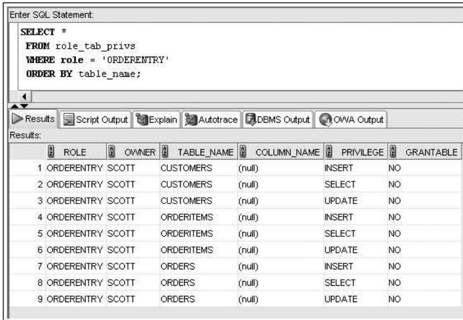
FIGURE 7-24 Verifying privileges assigned to a role
