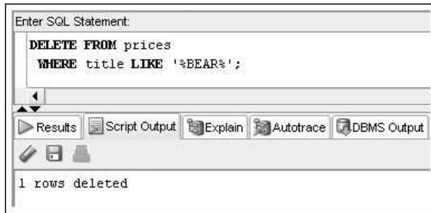
FIGURE 13-20 Deleting a book via the PRICES view
