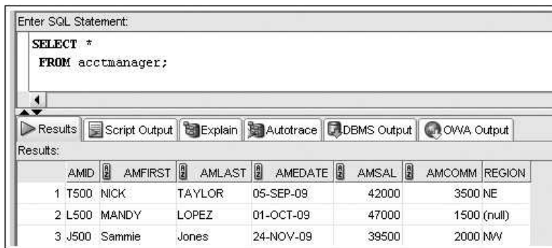
FIGURE 5-10 Contents of the ACCTMANAGER table
