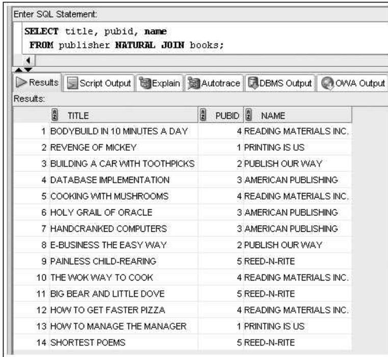
FIGURE 9-12 Using the NATURAL JOIN keywords
