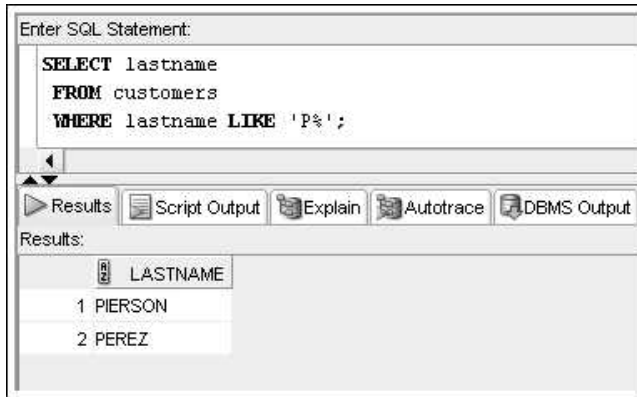
FIGURE 8-19 Searching with the LIKE operator and the % wildcard character
