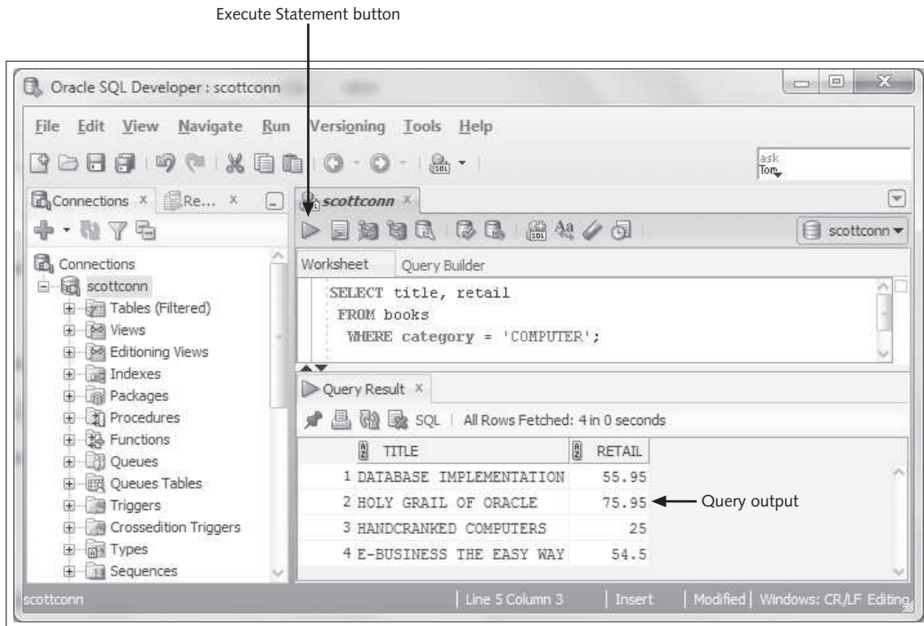
FIGURE B-7 Executing a query in SQL Developer
