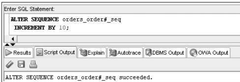
FIGURE 6-14 Command to change the INCREMENT BY setting for a sequence
