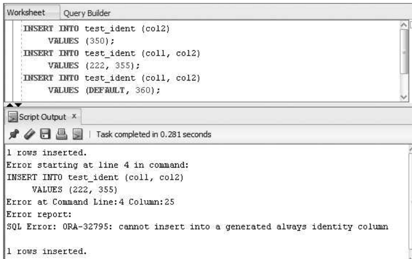
FIGURE 6-22 Test inserts on Identity Column
