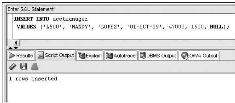
FIGURE 5-6 The INSERT INTO command for Mandy Lopez
