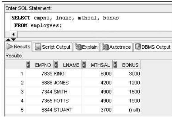
FIGURE 11-6 Data in the EMPLOYEES table
