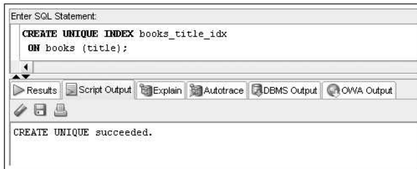
FIGURE 6-28 Explicitly creating a unique index
