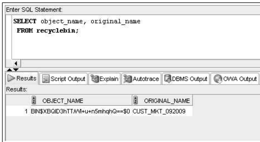
FIGURE 3-40 Checking the recycle bin
