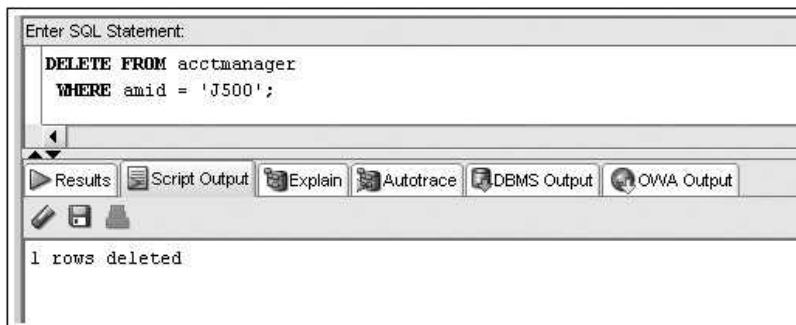
FIGURE 5-32 DELETE command to remove a row from the ACCTMANAGER table
