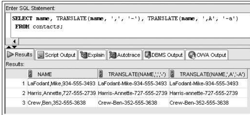
FIGURE 10-14 Using TRANSLATE to substitute character values
