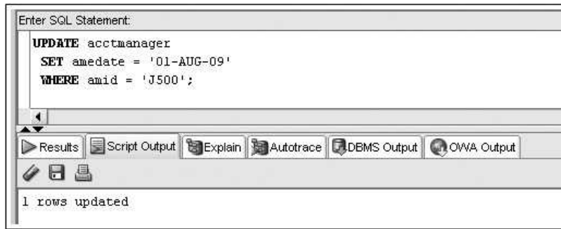
FIGURE 5-24 Command to correct the Amedate column value
