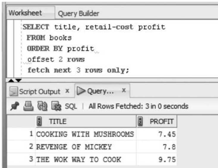
FIGURE 13-35 Offset option to skip rows
