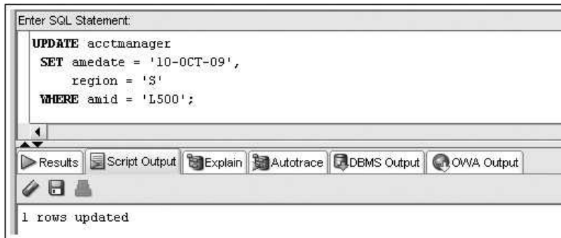
FIGURE 5-26 Updating multiple columns
