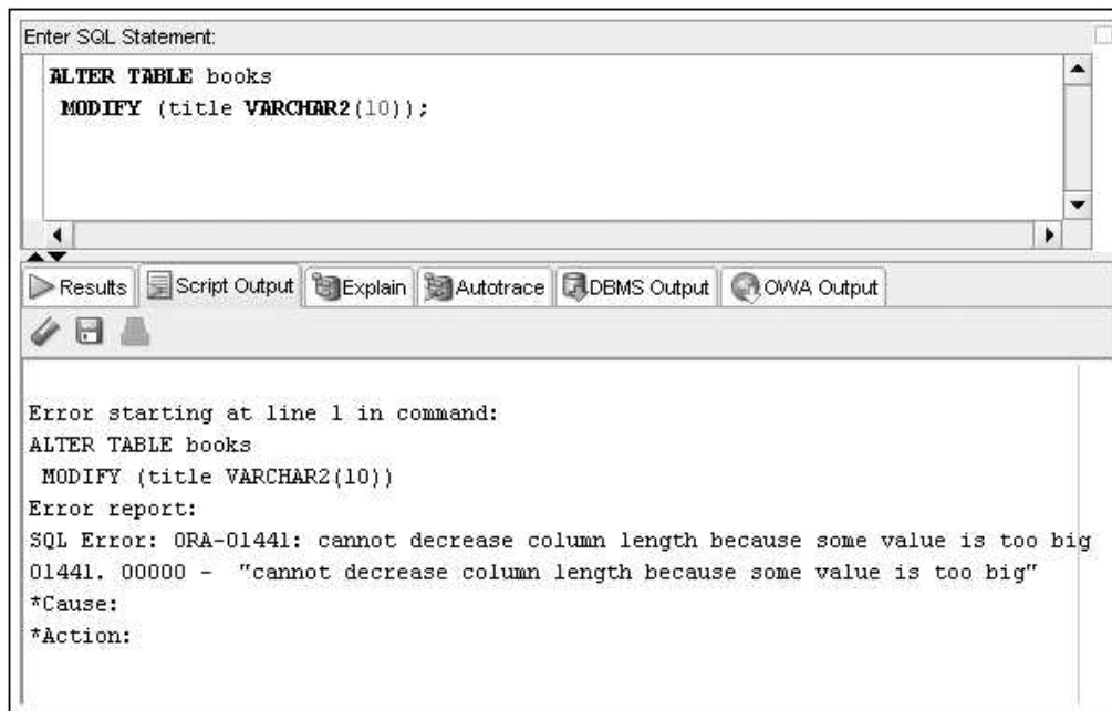
FIGURE 3-18 Modify column size error
