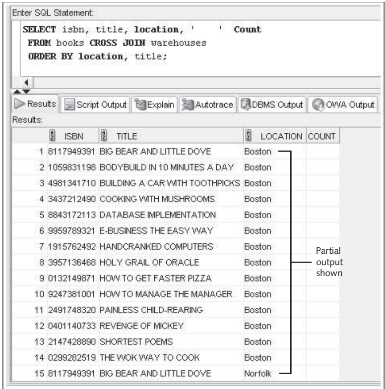
FIGURE 9-4 Using the CROSS JOIN keywords
