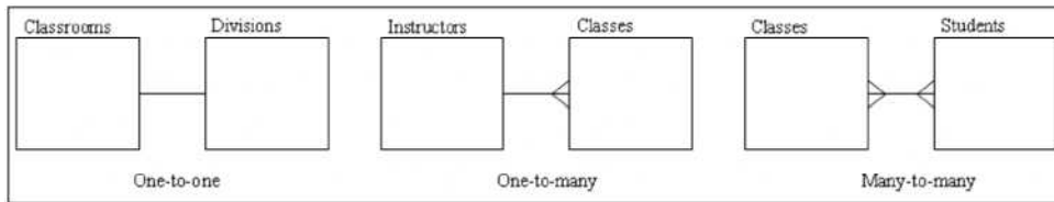
FIGURE 1-3 E-R model notation examples
