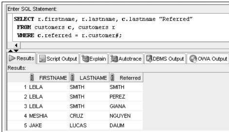
FIGURE 9-22 A self-join with the traditional method
