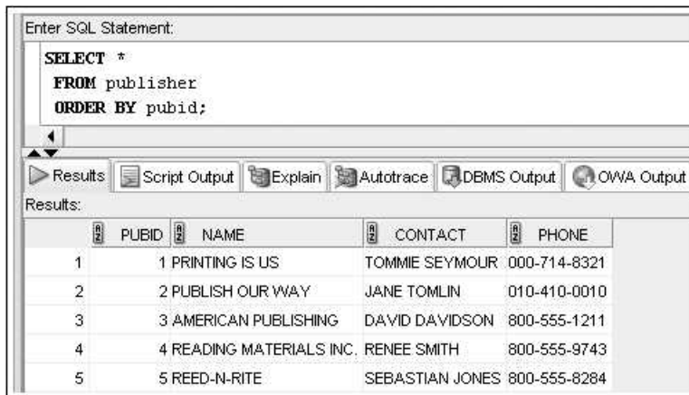
FIGURE 9-34 The PUBLISHER table
