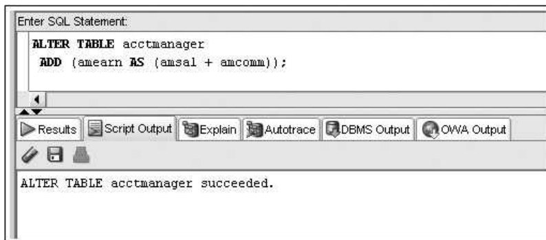
FIGURE 5-13 Add a virtual column
