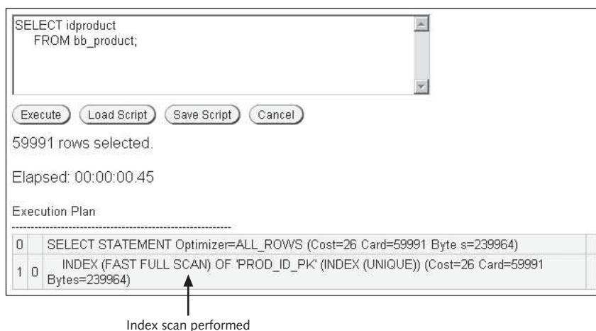
FIGURE E-8 Explain plan and execution time for the modified query
