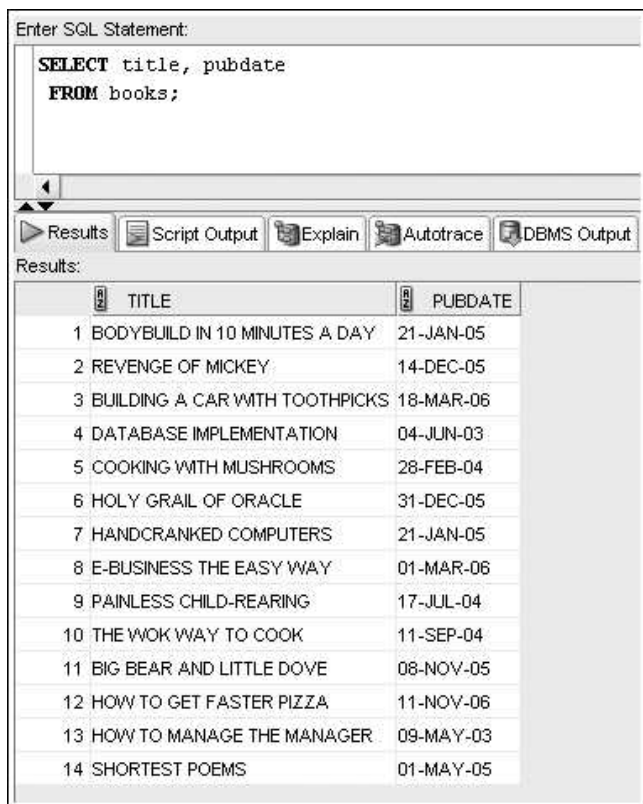
FIGURE 2-9 Command to select multiple columns from a table
