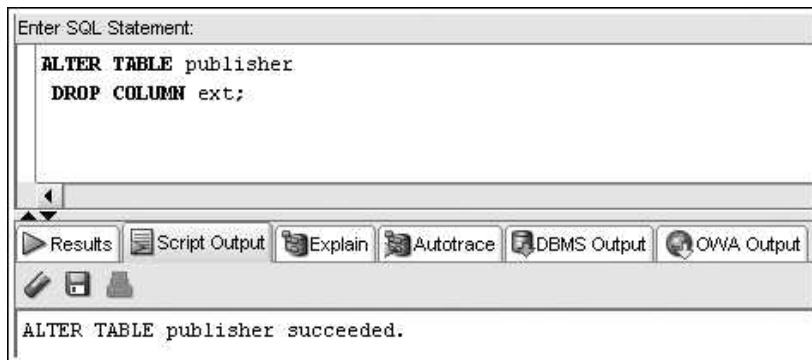
FIGURE 3-24 The ALTER TABLE ... DROP COLUMN command
