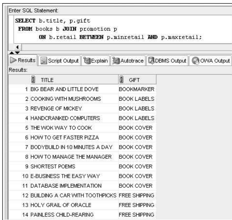
FIGURE 9-20 The JOIN method for a non-equality join
