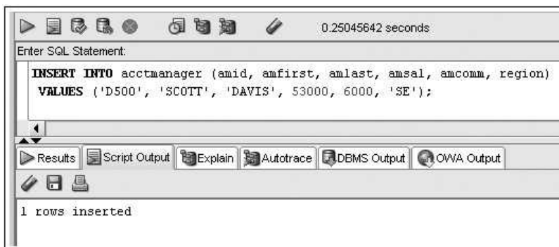
FIGURE 5-16 Successful INSERT on a table with a virtual column
