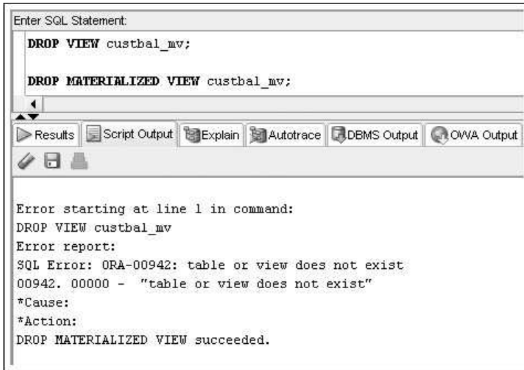
FIGURE 13-38 Drop a materialized view
