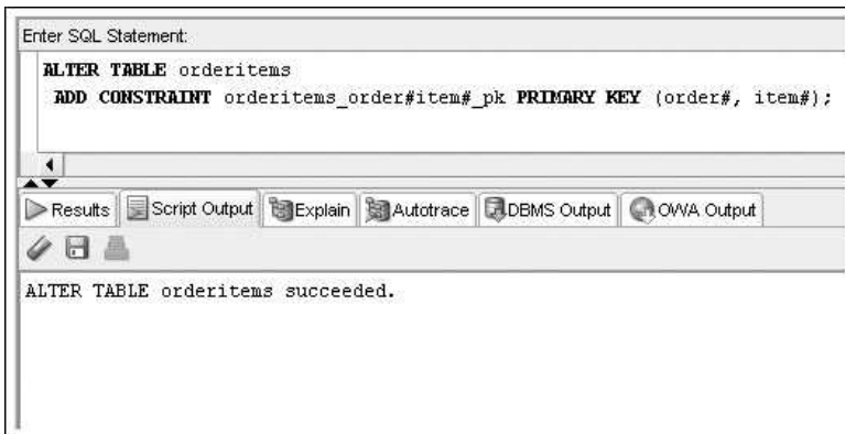
FIGURE 4-7 Adding a composite PRIMARY KEY constraint
