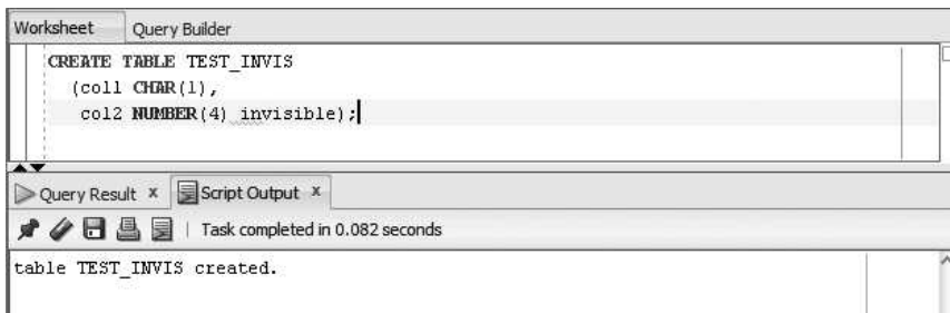
FIGURE 3-6 Define an invisible column
