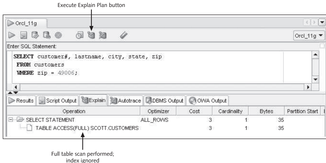
FIGURE 6-26 View the explain plan indicating a full table scan
