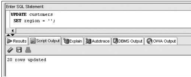
FIGURE 5-27 Clear the Region column
