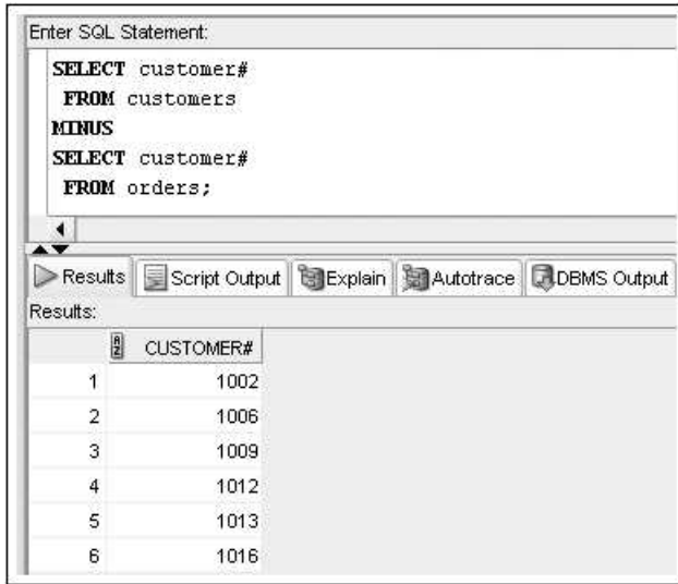
FIGURE 9-38 Subtract result sets with the MINUS set operator
