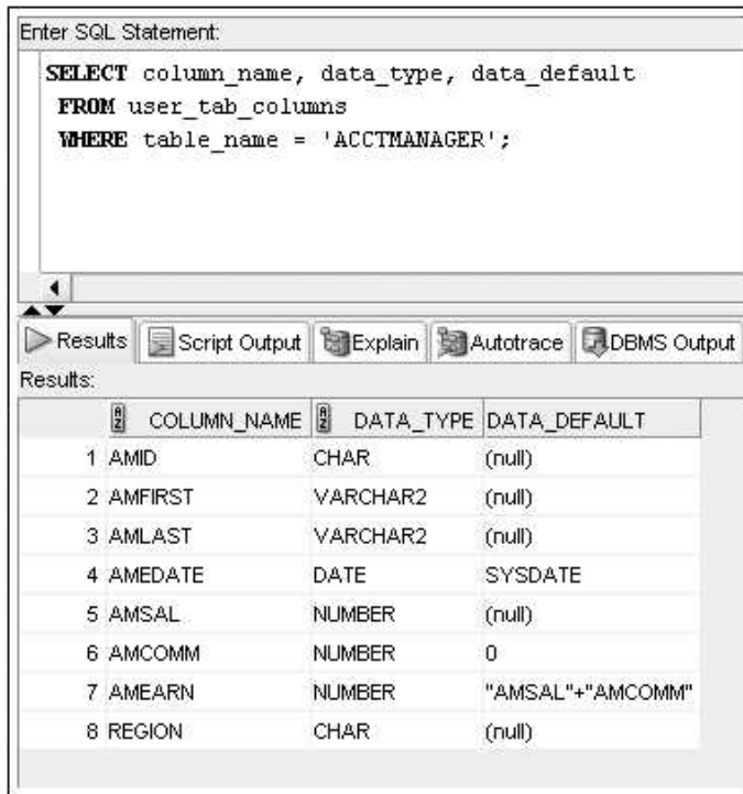
FIGURE 3-5 Verify DEFAULT and virtual column settings
