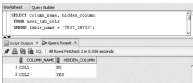
FIGURE 3-9 Use the data dictionary to identify invisible columns
