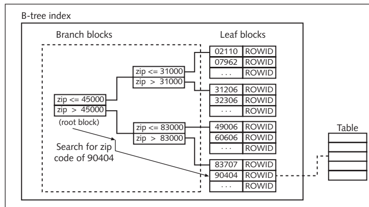
FIGURE 6-25 B-tree index organization
