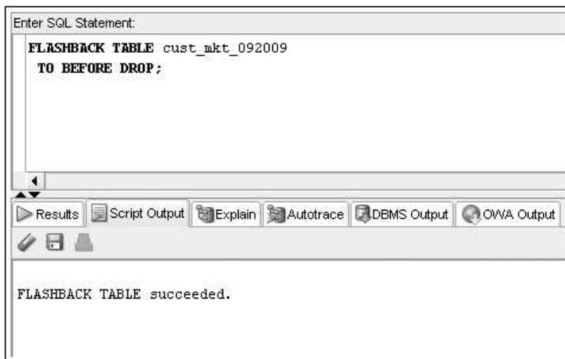
FIGURE 3-41 Using FLASHBACK TABLE to restore a dropped table
