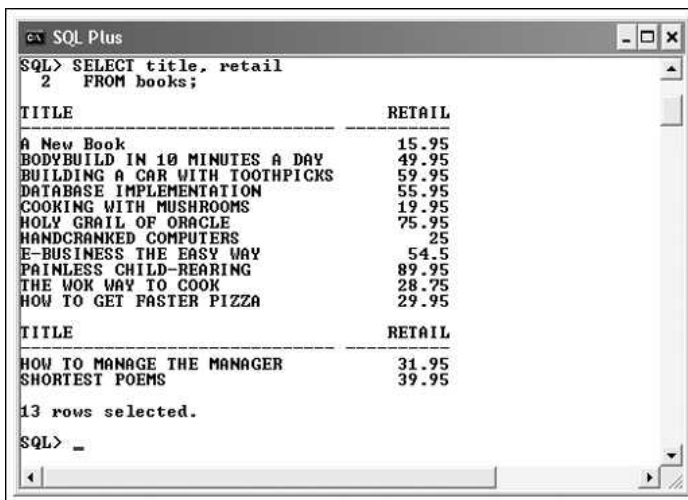
FIGURE B-2 Executing a query in SQL*Plus
