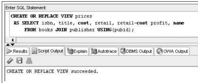
FIGURE 13-17 PRICES view with a table join
