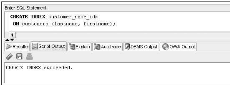
FIGURE 6-30 Creating a composite index
