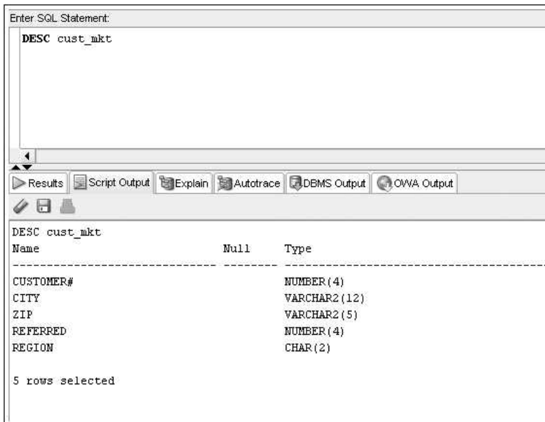
FIGURE 3-28 Verifying that the column is no longer available
